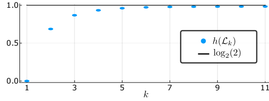
Figure 5.5: Evolution of h(\mathcal{L}_k) of Example 5.4.2 in terms of k .
