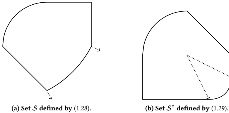
Figure 1.3: Illustration for sets \mathcal{S} and \mathcal{S}^\circ defined in Example 1.4.2.
