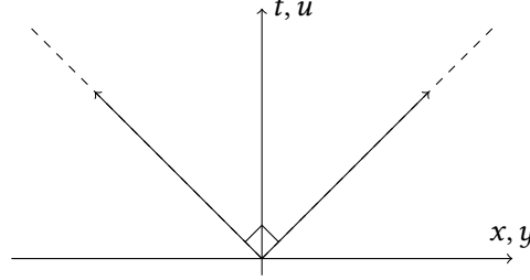
Figure 2.1: Visualization of second order cone and complementarity slackness. If (t, x), (u, y) belong to the second-order cone and (t, x) \cdot (u, y) = 0 , then (u, y) is parallel to (t, -x) or (t, x) is zero or (u, y) is zero.
