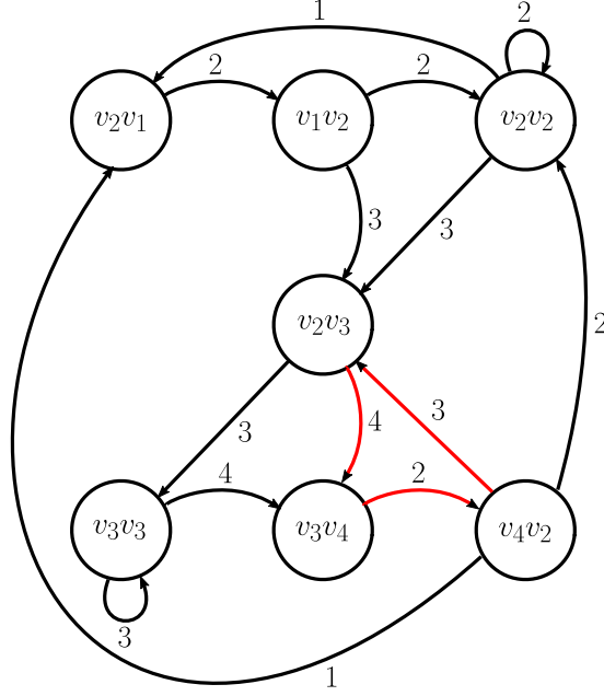
Figure 5.7: Second degree lifted automaton of Example 5.4.3.
