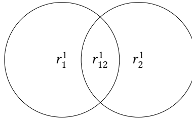
Figure 7.2: The decomposition of an entropy vector of 2 variables in its atoms.
