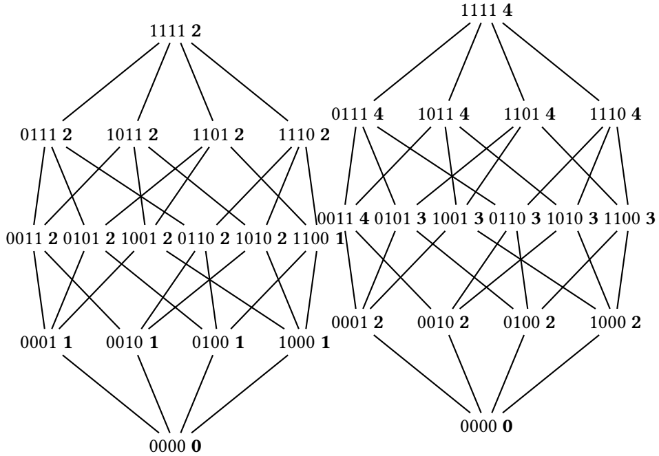
(c) X_1 and X_2 are independent coin tosses free expansion is the Vamos matroid and X_4 = X_3 = X_1 \oplus X_2 . (d) Non-entropic extreme ray of \mathcal{P}_4 . Its free expansion is the Vamos matroid [Vam68].
