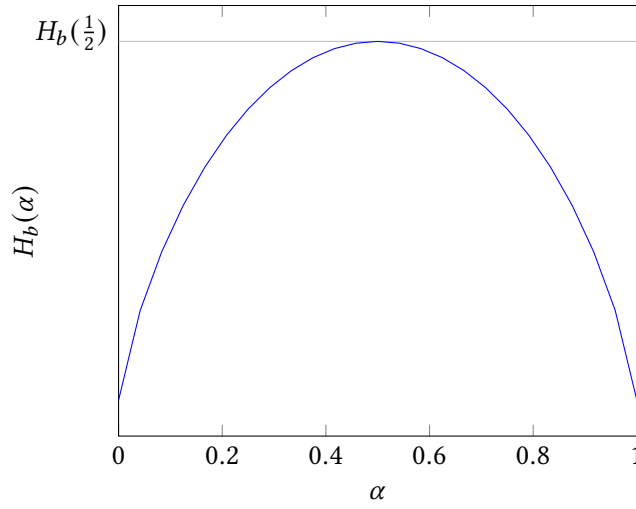
Figure 7.1: The value of H_b(\alpha) for 0 \leq \alpha \leq 1 .
